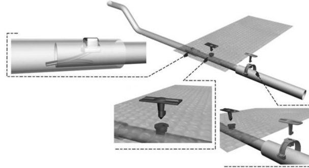
Fig 2 - Parts Assembly
